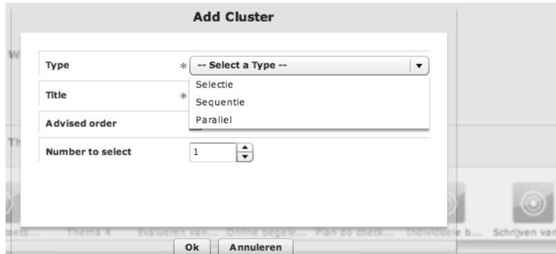
Figure 5.6. Learning Path Editor Design view: Add Cluster
