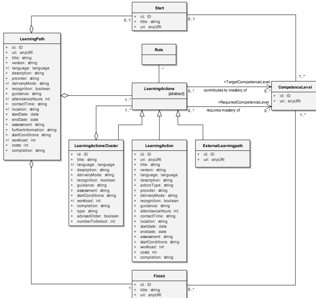
Figure 1. LearningPath conceptual model
