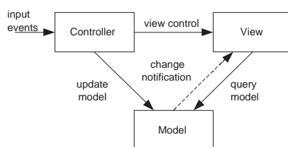
FIGURE 3.13 Model-View-Controller
