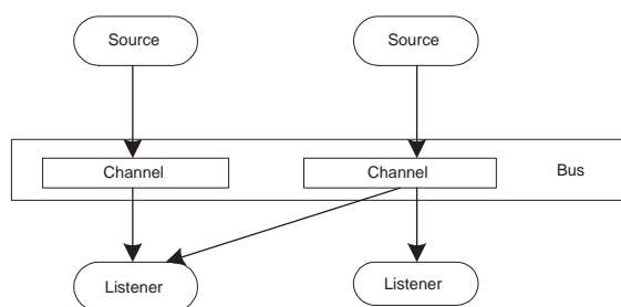
FIGURE 3.11 Event-Bus pattern
